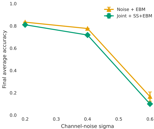
Noise robustness: CART (IID)
