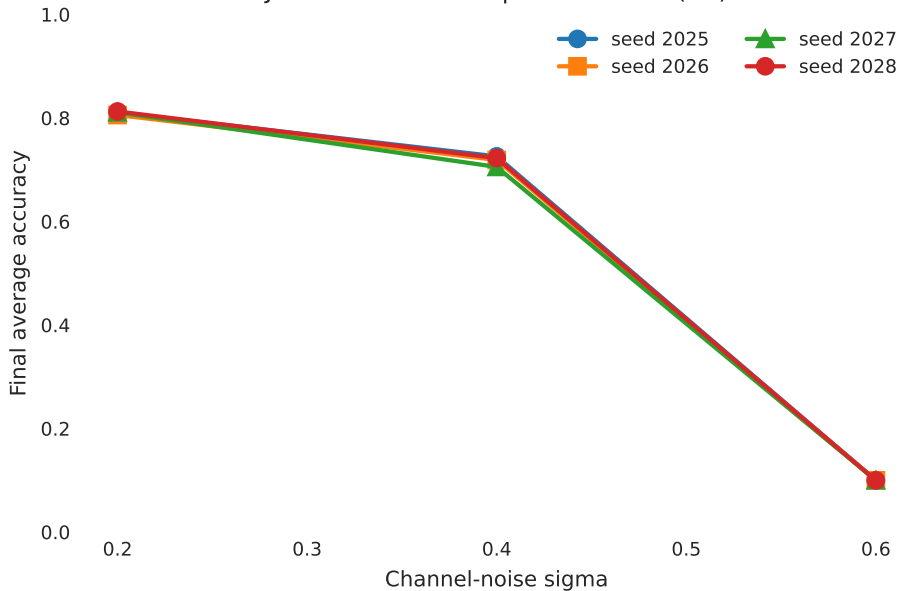
Joint SS+EBM seed profiles: CART (IID)
