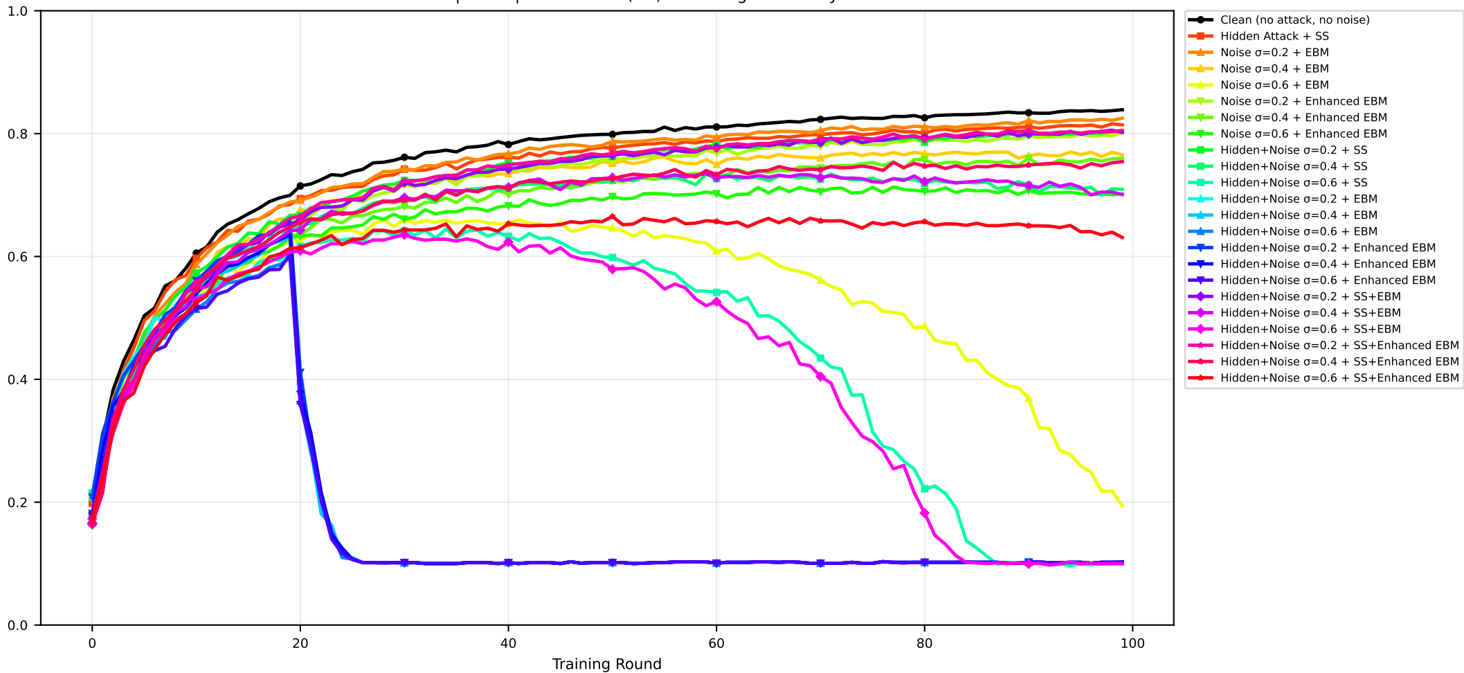
CIFAR-10 | CART | seed=2027 (IID) — Average Accuracy
