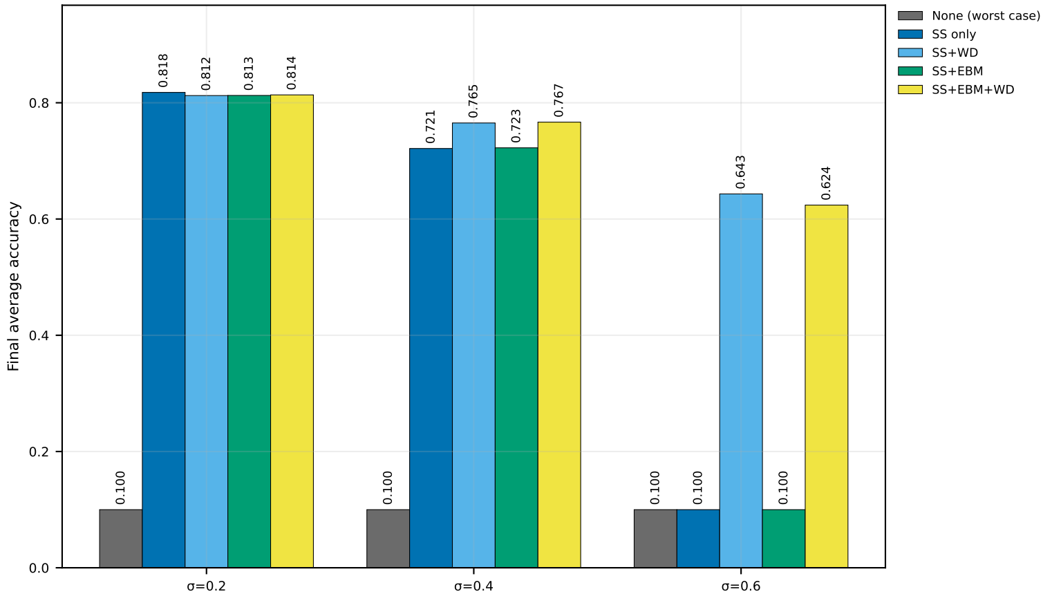
Ablation Groups (Byzantine Attack) | CIFAR-10 | CART | seed=2028 (IID)
