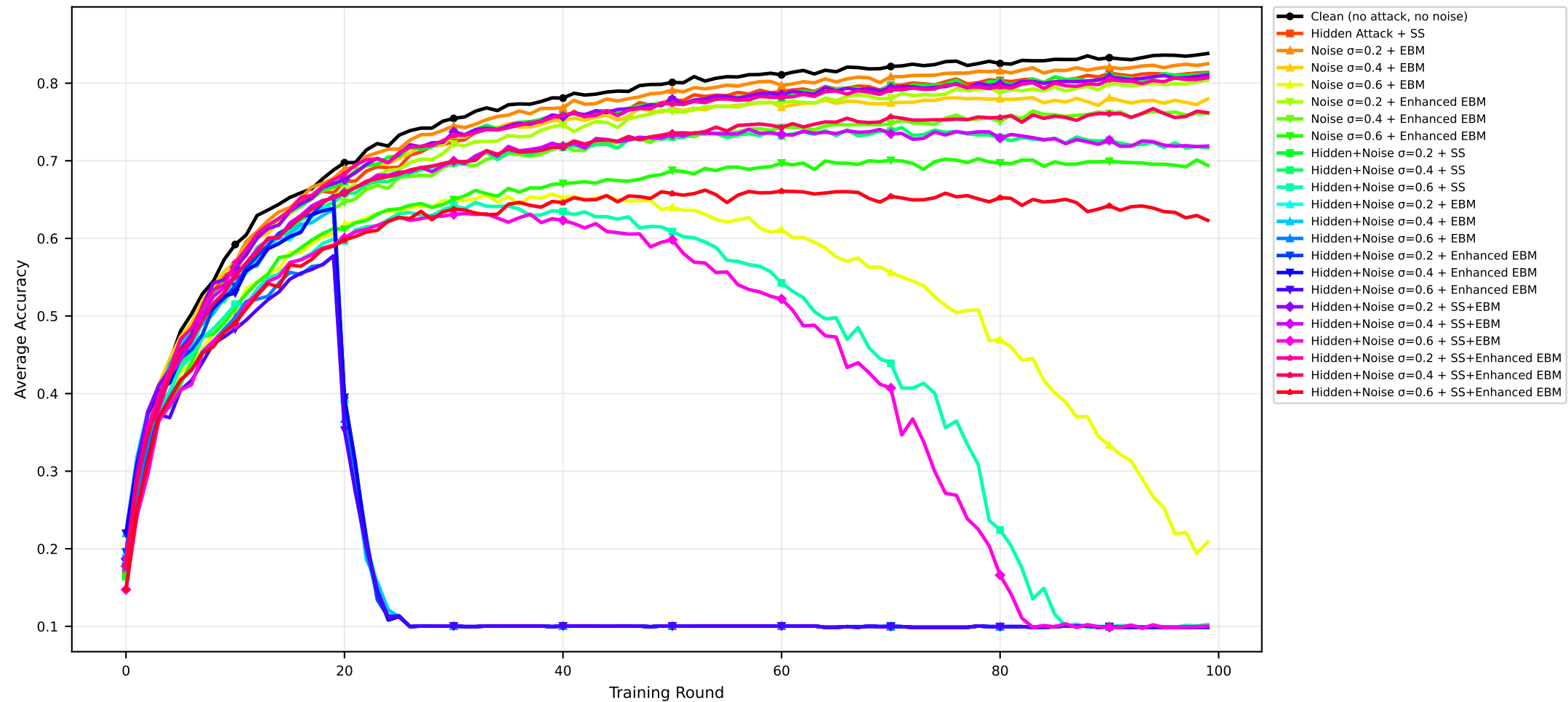
Zoomed Accuracy | CIFAR-10 | CART | seed=2028 (IID)
