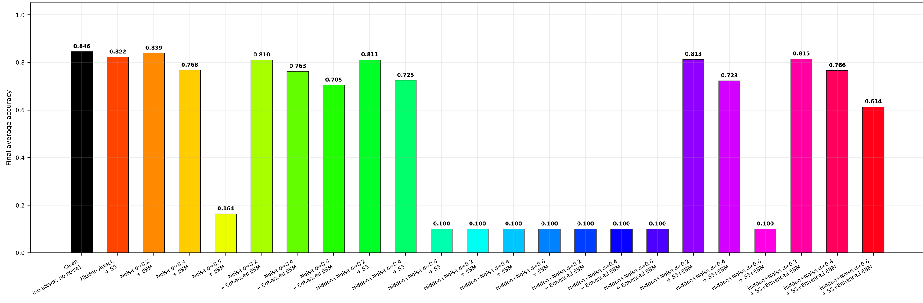
Final Accuracy | CIFAR-10 | MERGED | seed=2027 (IID)
