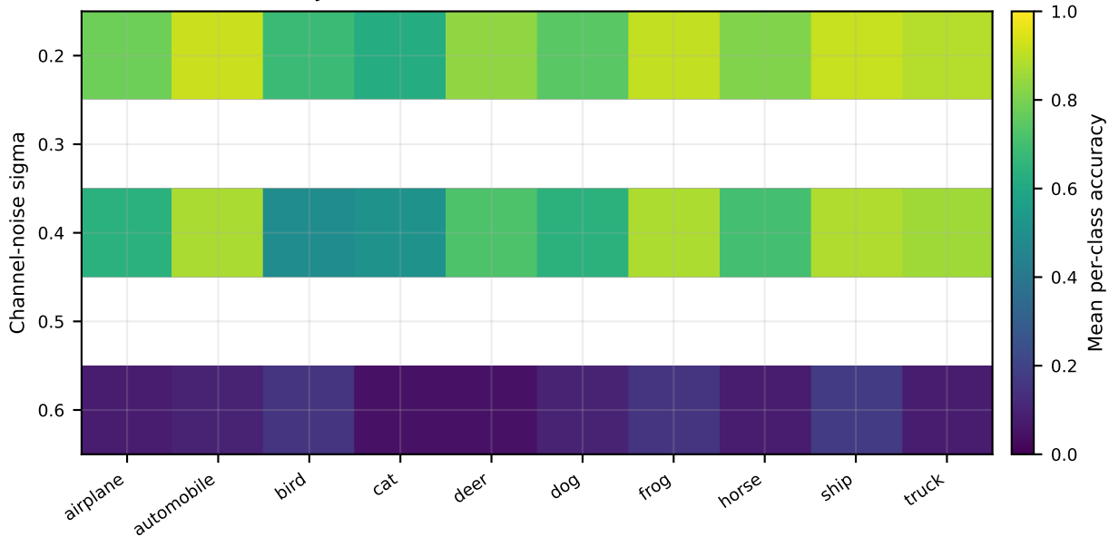
Joint SS+EBM class retention: CART (IID)
