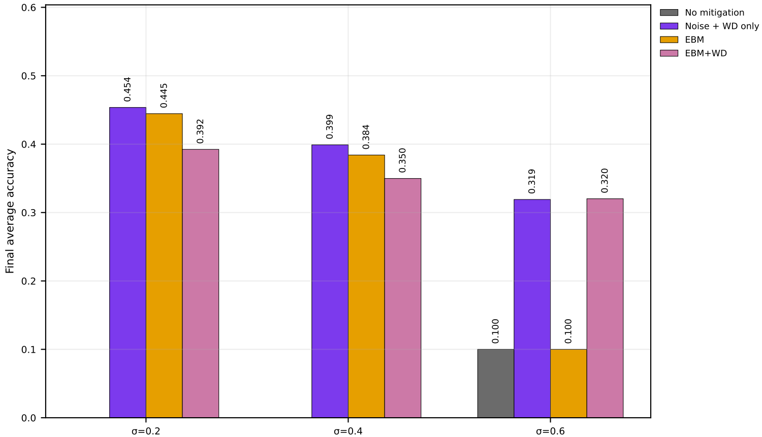
Ablation Groups (Channel Noise) | CIFAR-10 | CART | seed=2028 (nonIID)
