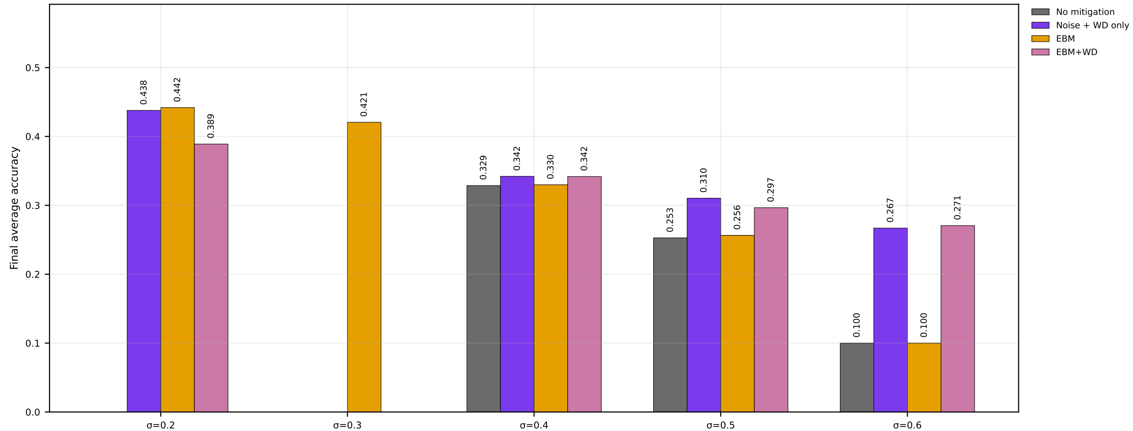
Ablation Groups (Channel Noise) | CIFAR-10 | MERGED | seed=2025 (nonIID)
