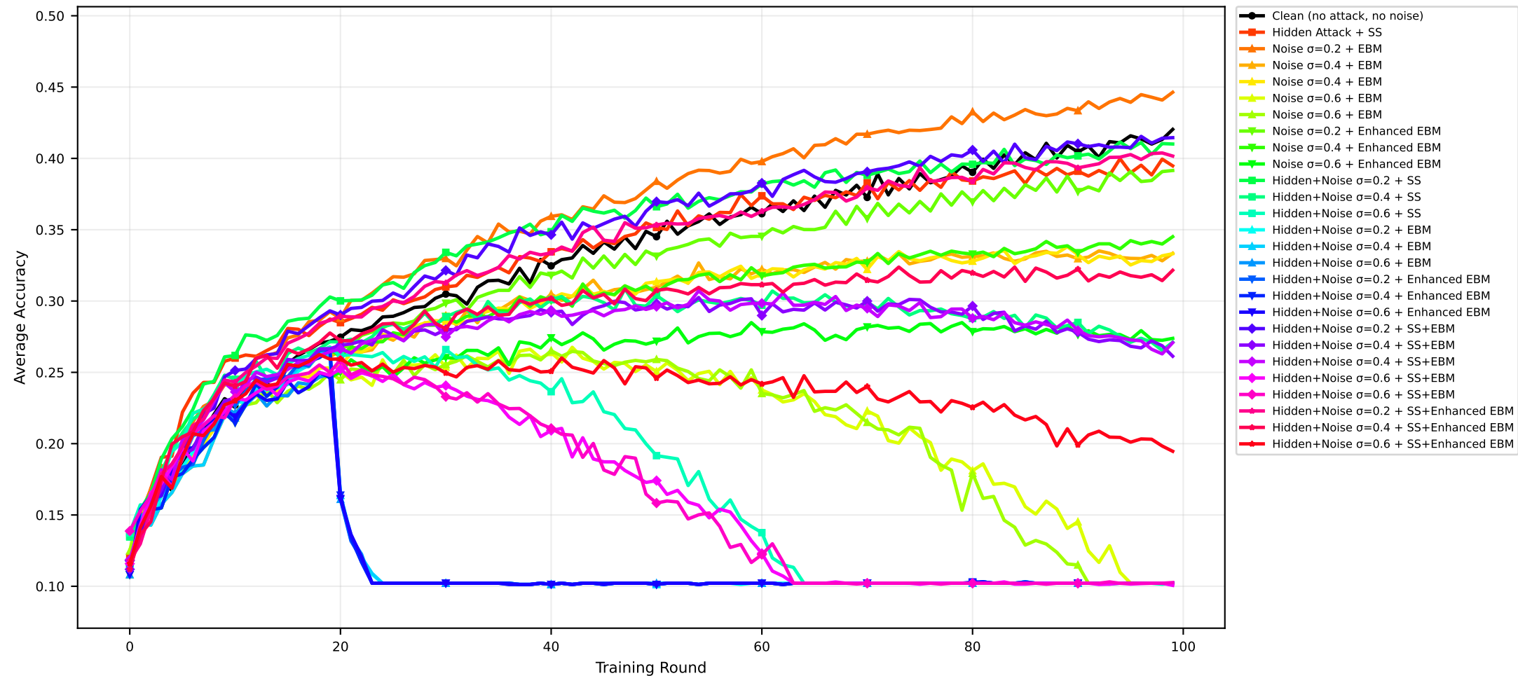
Zoomed Accuracy | CIFAR-10 | MERGED | seed=2025 (nonIID)
