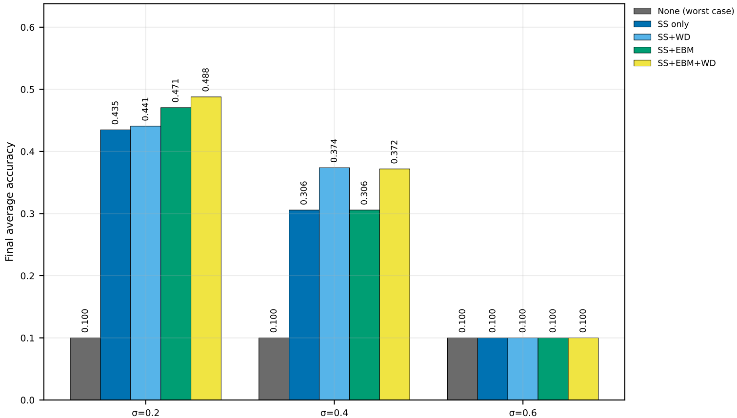
Ablation Groups (Byzantine Attack) | CIFAR-10 | MERGED | seed=2027 (nonIID)
