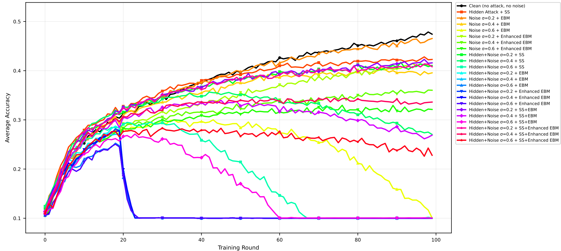
Zoomed Accuracy | CIFAR-10 | MERGED | seed=2028 (nonIID)
