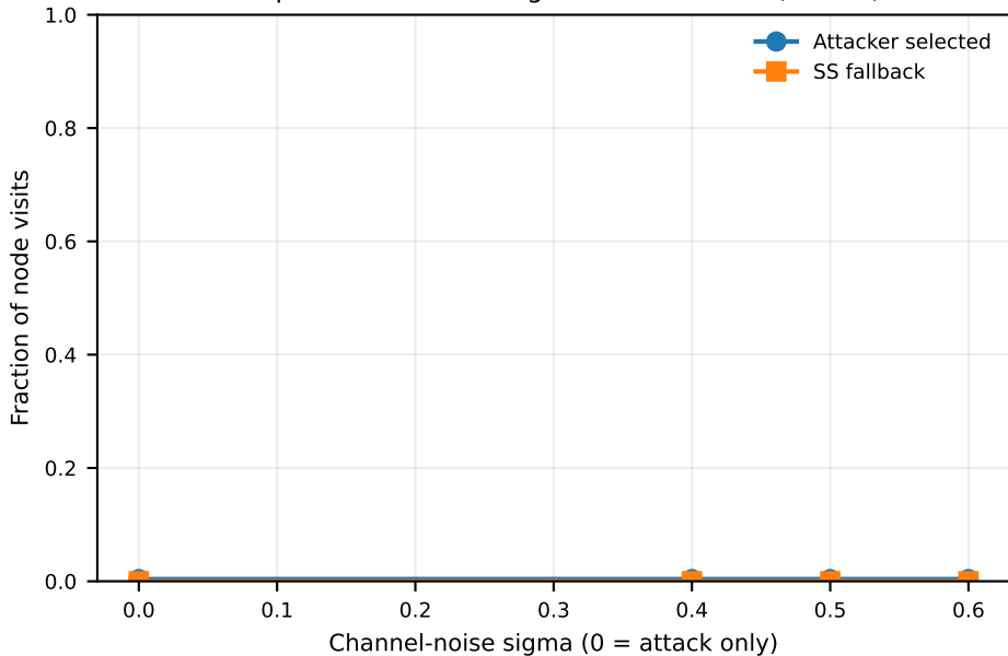
Snapshot Selection diagnostics: MERGED (nonIID)
