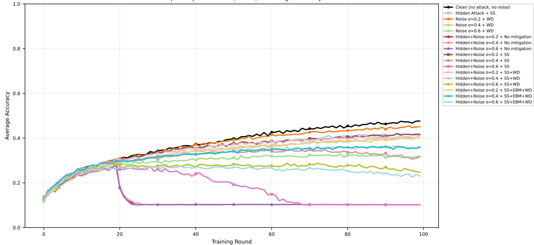
CIFAR-10 | CART | seed=2025 (nonIID) — Average Accuracy
