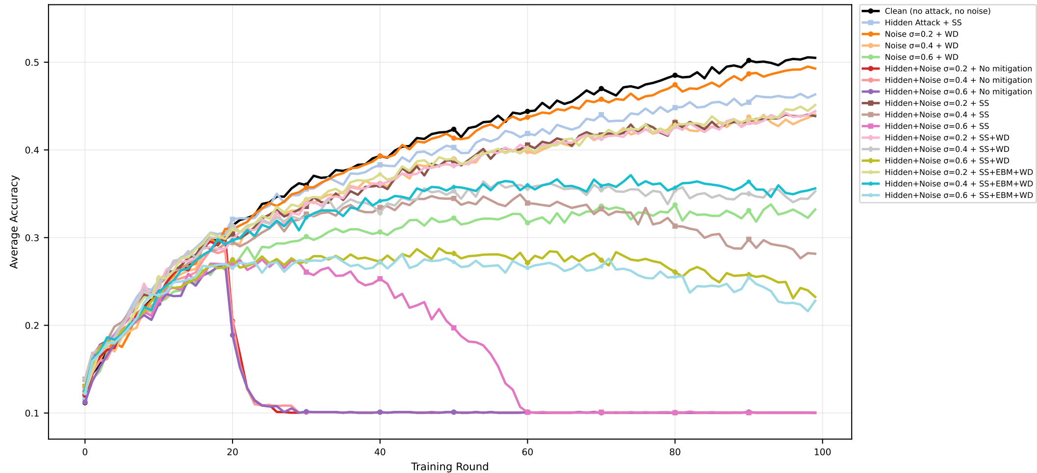
Zoomed Accuracy | CIFAR-10 | CART | seed=2026 (nonIID)
