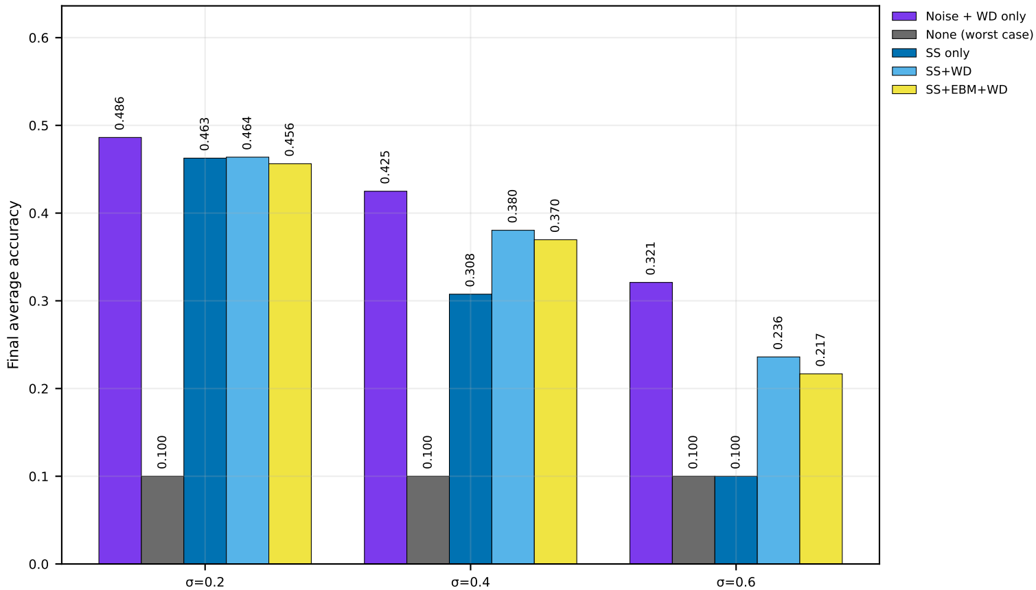
Ablation Groups | CIFAR-10 | CART | seed=2027 (nonIID)
