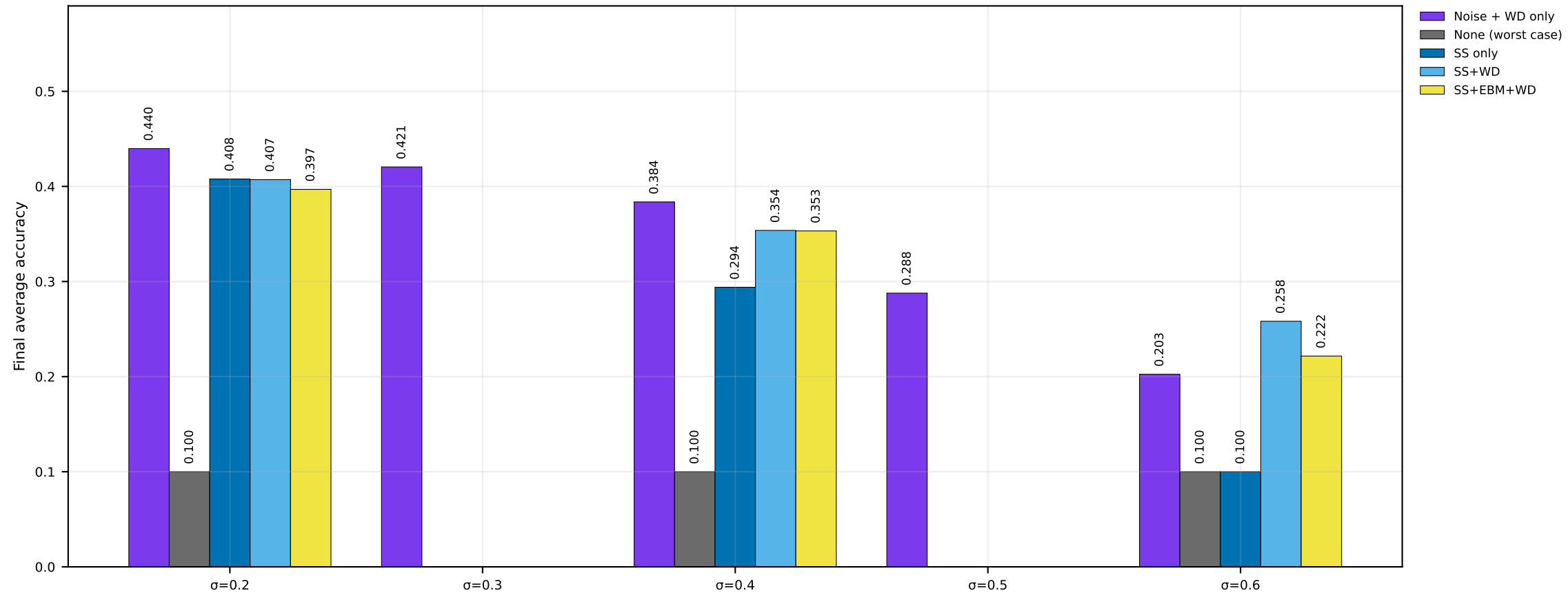
Ablation Groups | CIFAR-10 | MERGED | seed=2025 (nonIID)
