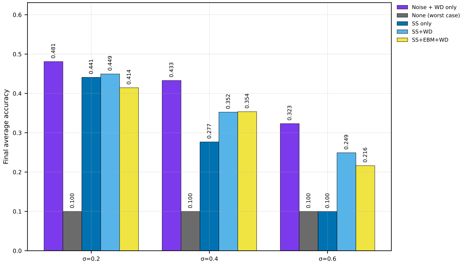
Ablation Groups | CIFAR-10 | MERGED | seed=2026 (nonIID)
