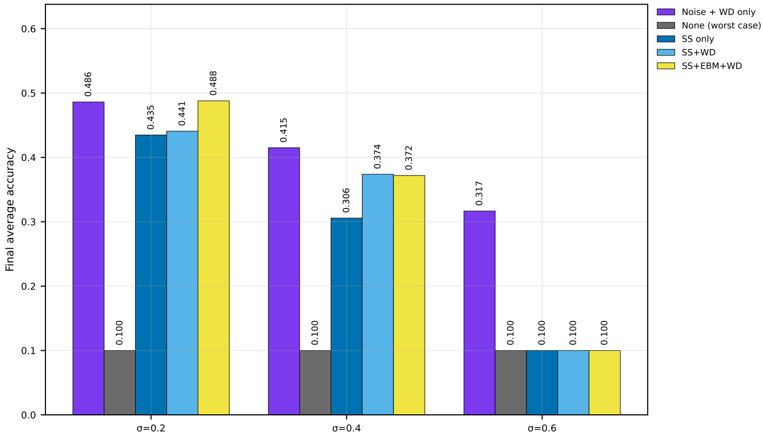
Ablation Groups | CIFAR-10 | MERGED | seed=2027 (nonIID)
