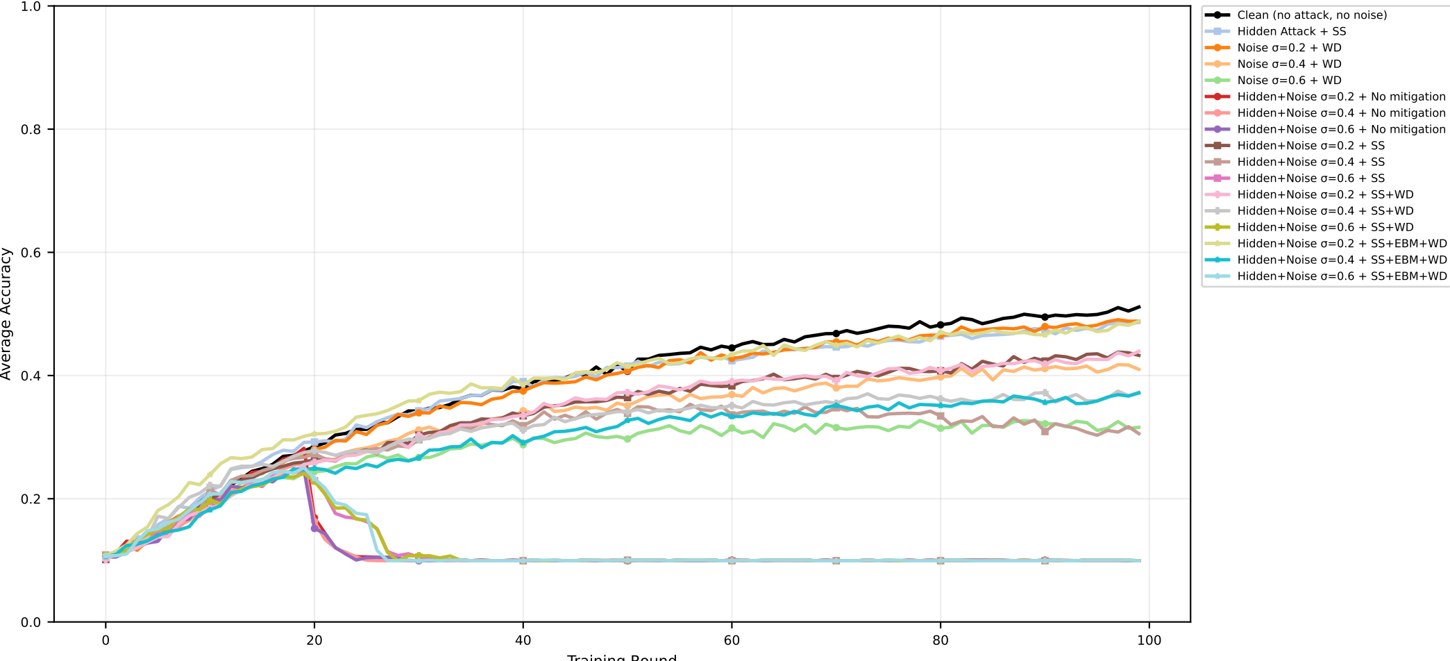
CIFAR-10 | MERGED | seed=2027 (nonIID) — Average Accuracy
