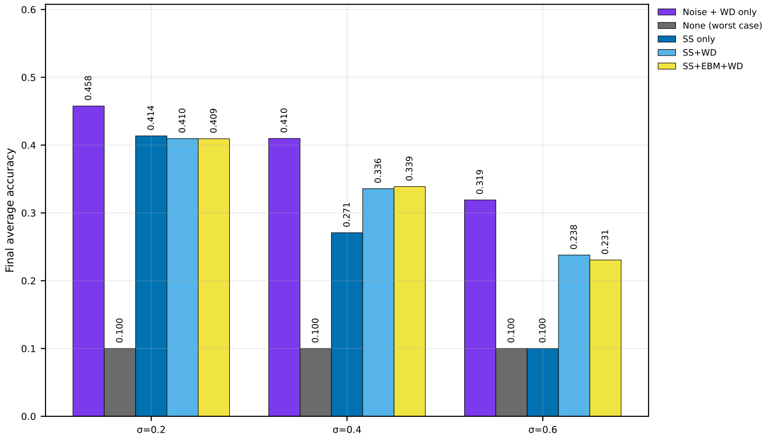
Ablation Groups | CIFAR-10 | MERGED | seed=2028 (nonIID)
