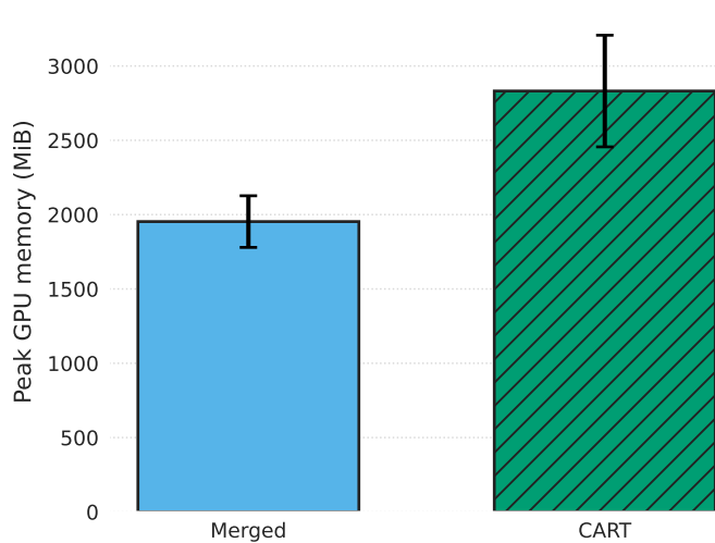
(b) TensorFlow peak allocation
