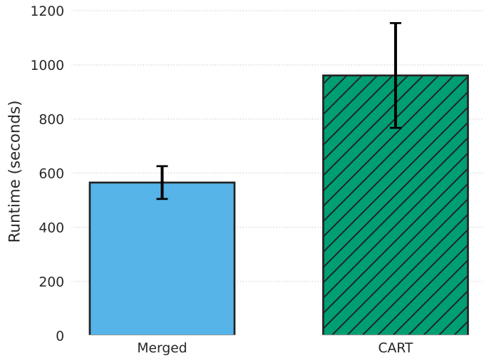
(a) Wall-clock runtime
