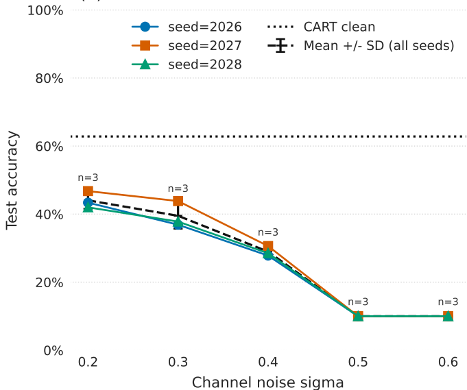
(b) Hidden attack + channel noise + SS+EBM
