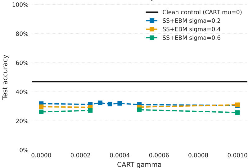
CART calibration by noise level
