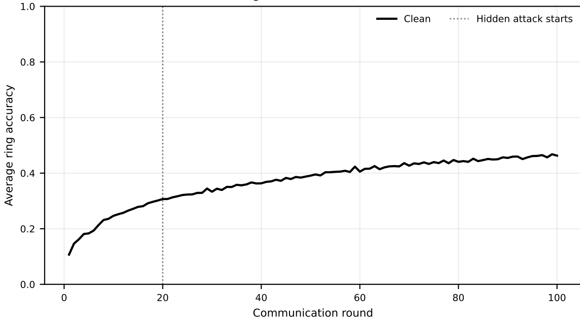
Learning curves: MERGED (nonIID)
