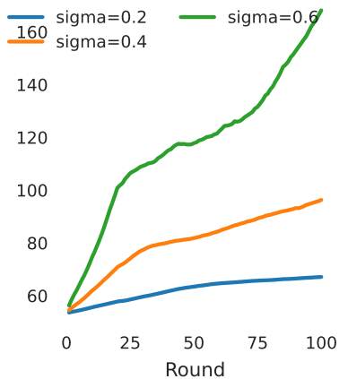
Consensus innovation
