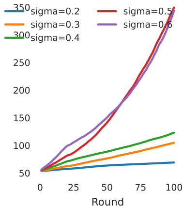
Consensus innovation
