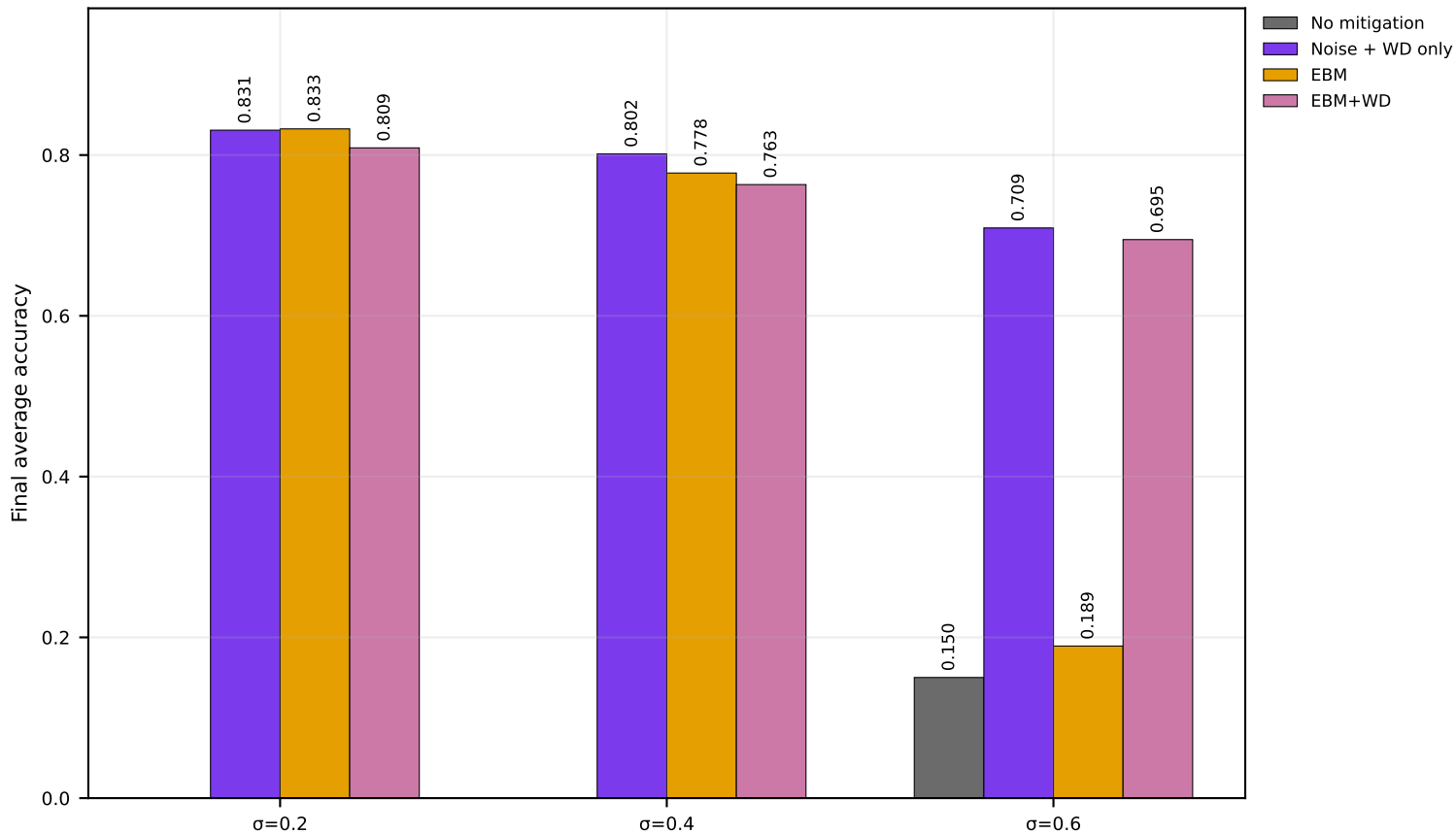
Ablation Groups (Channel Noise) | CIFAR-10 | CART | seed=2025 (IID)
