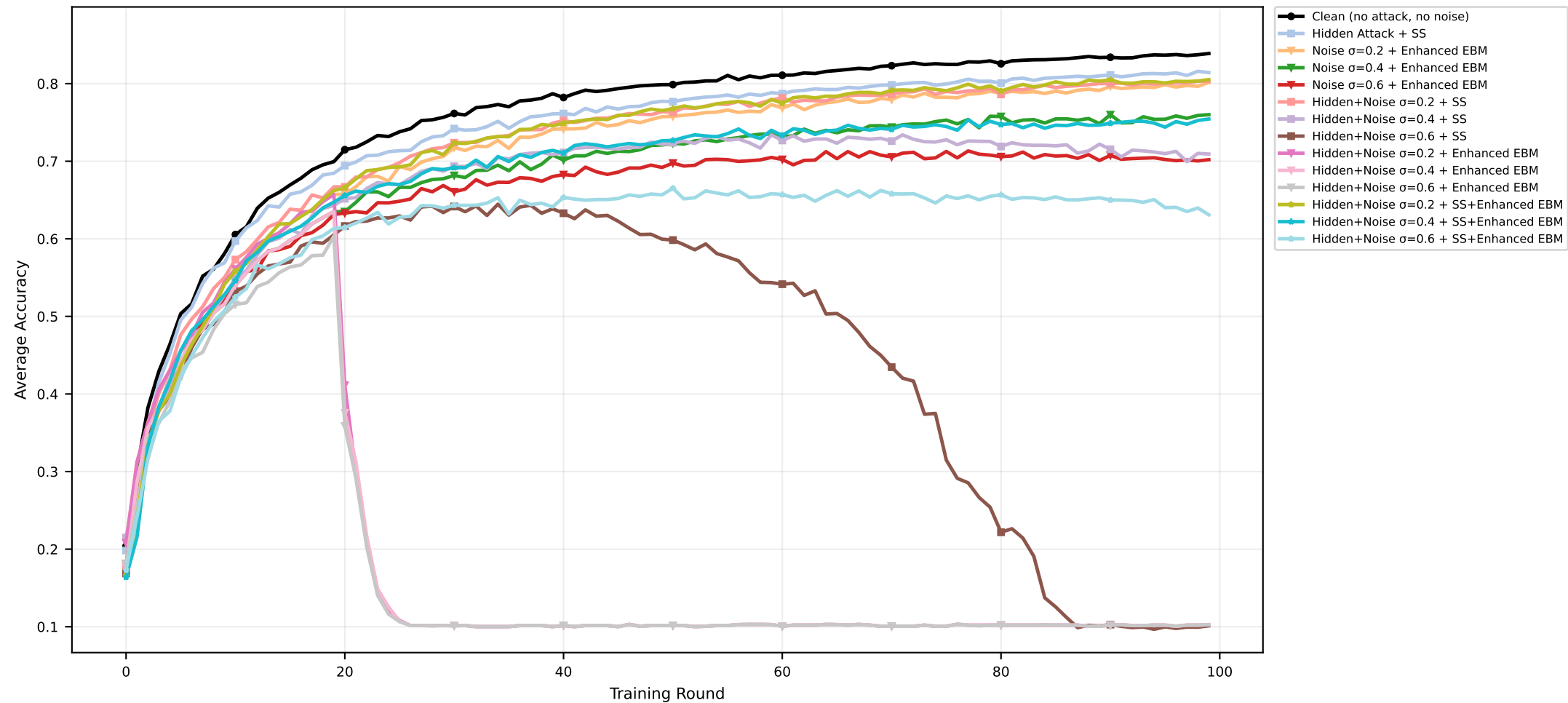
Zoomed Accuracy | CIFAR-10 | CART | seed=2027 (IID)
