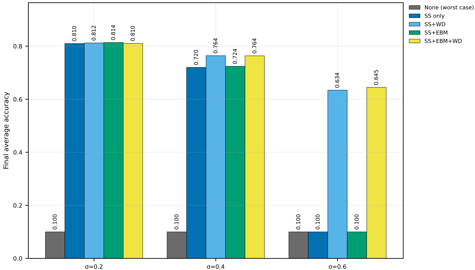
Ablation Groups (Byzantine Attack) | CIFAR-10 | MERGED | seed=2025 (IID)
