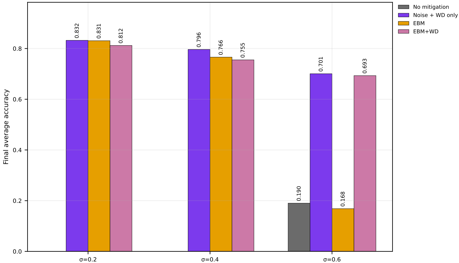
Ablation Groups (Channel Noise) | CIFAR-10 | MERGED | seed=2028 (IID)
