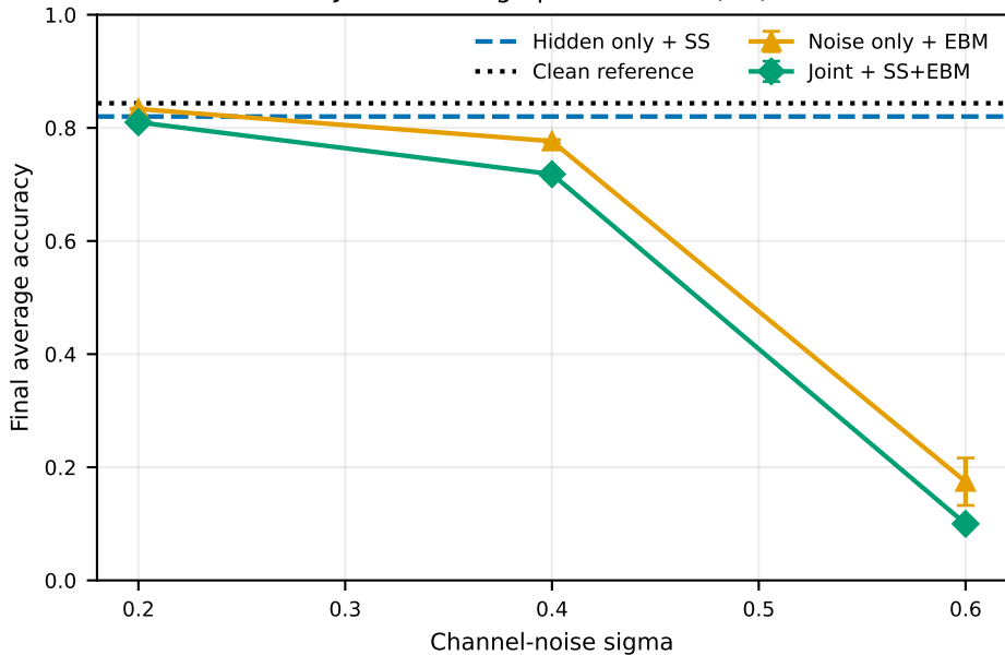
Joint challenge profile: CART (IID)
