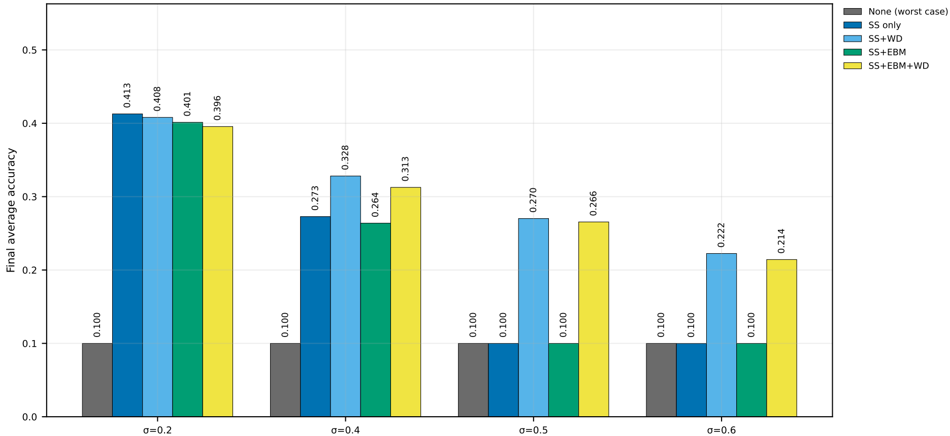
Ablation Groups (Byzantine Attack) | CIFAR-10 | CART | seed=2025 (nonIID)
