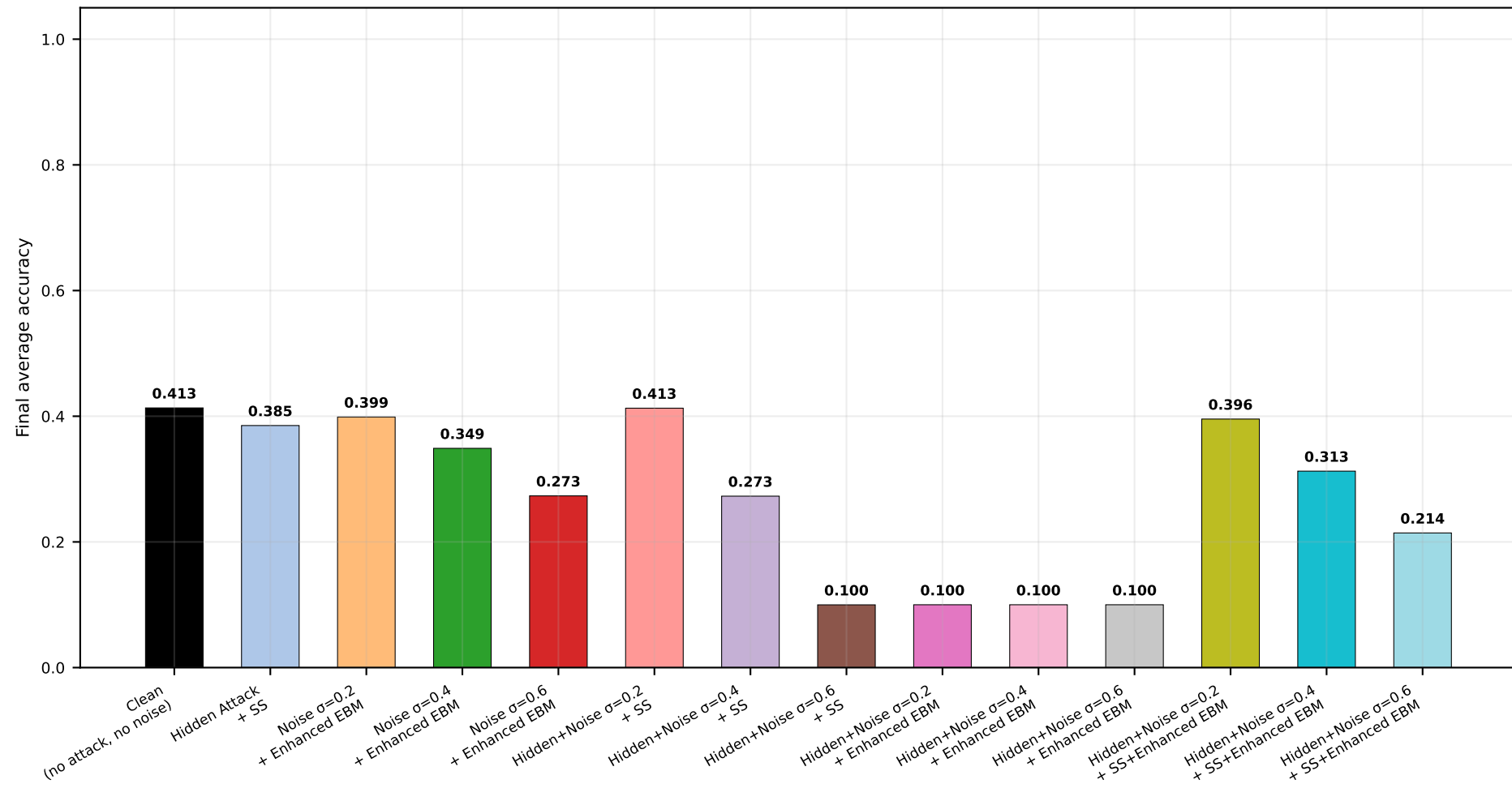
Final Accuracy | CIFAR-10 | CART | seed=2025 (nonIID)
