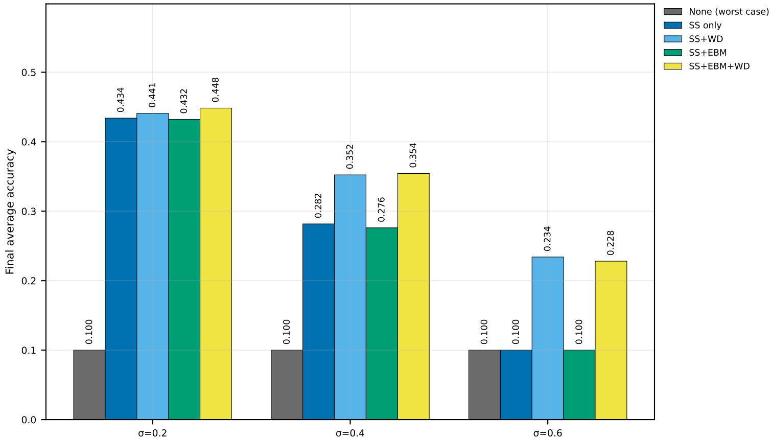
Ablation Groups (Byzantine Attack) | CIFAR-10 | CART | seed=2026 (nonIID)
