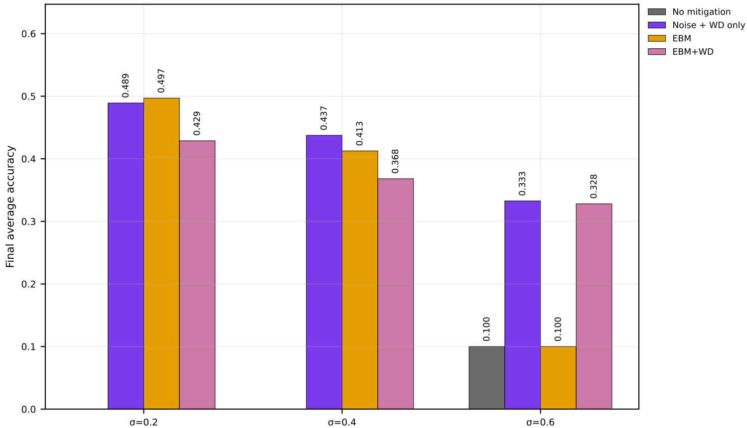
Ablation Groups (Channel Noise) | CIFAR-10 | CART | seed=2026 (nonIID)
