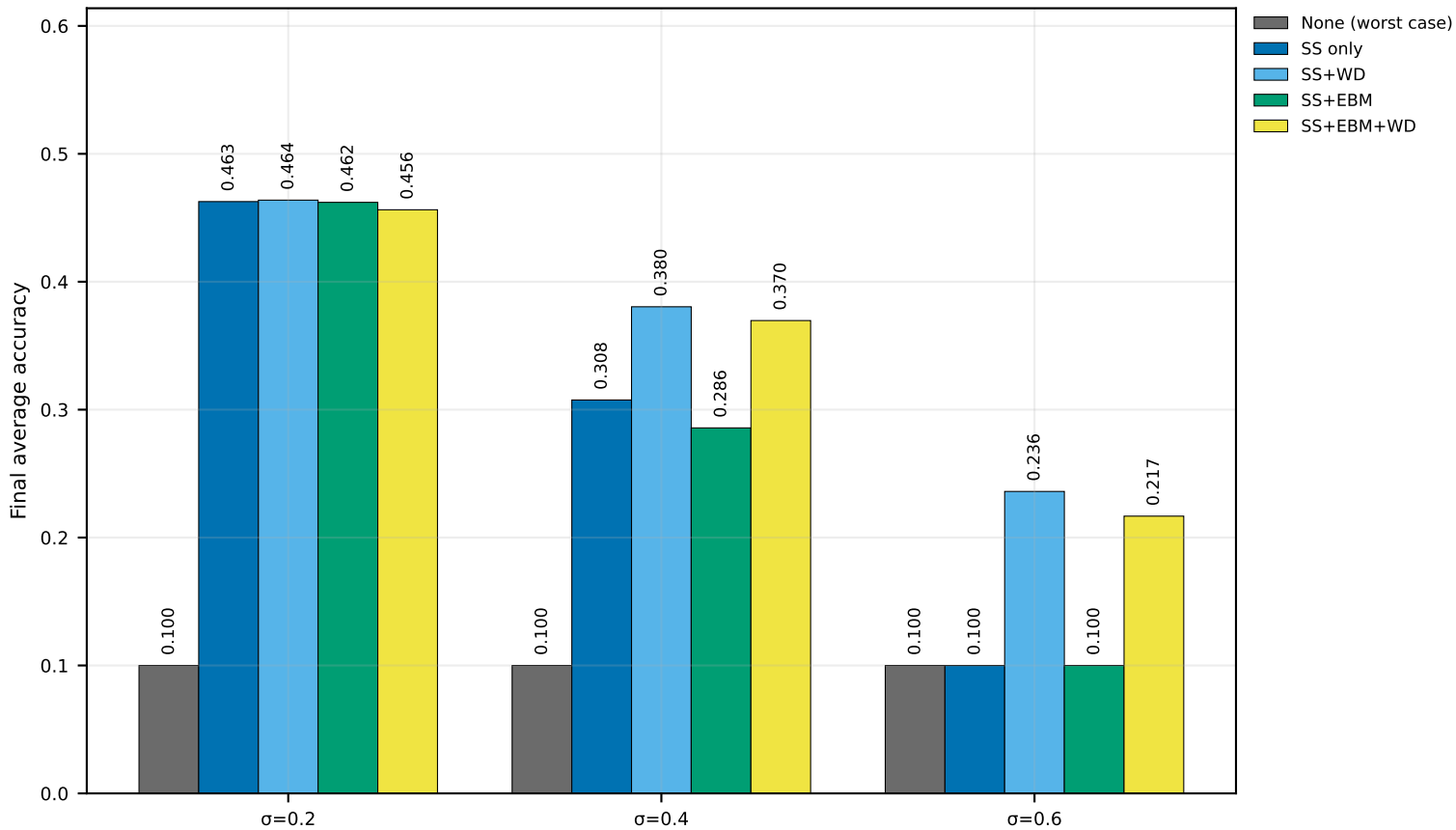
Ablation Groups (Byzantine Attack) | CIFAR-10 | CART | seed=2027 (nonIID)
