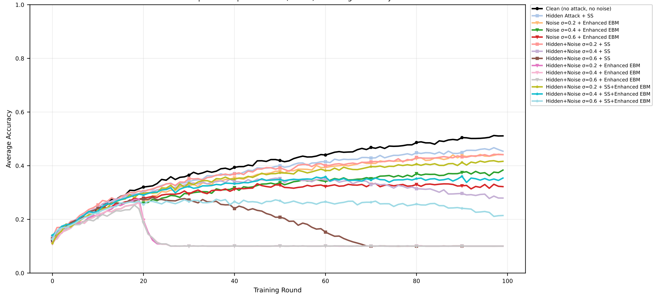
CIFAR-10 | MERGED | seed=2026 (nonIID) — Average Accuracy
