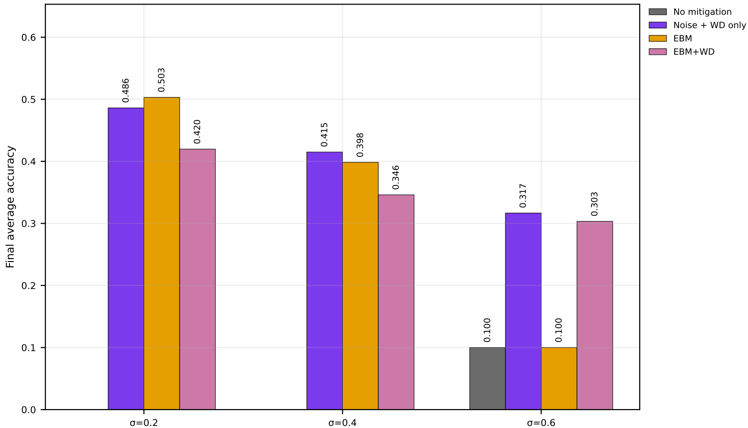
Ablation Groups (Channel Noise) | CIFAR-10 | MERGED | seed=2027 (nonIID)
