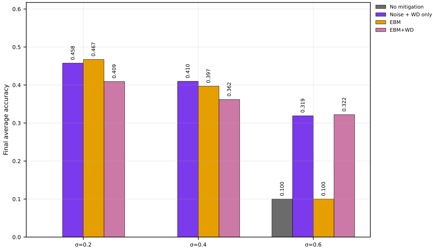
Ablation Groups (Channel Noise) | CIFAR-10 | MERGED | seed=2028 (nonIID)
