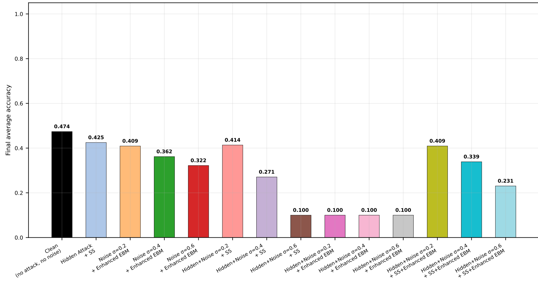
Final Accuracy | CIFAR-10 | MERGED | seed=2028 (nonIID)
