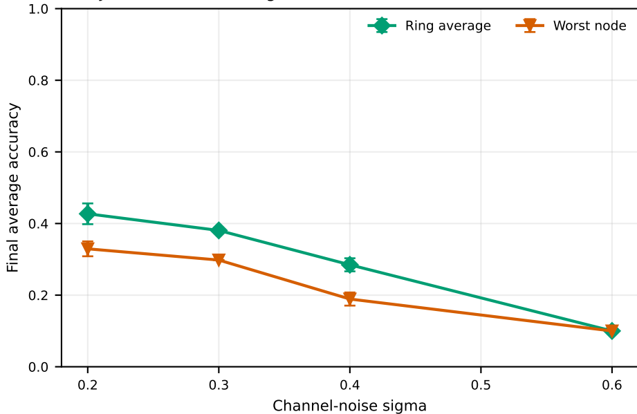
Joint SS+EBM average versus worst node: MERGED (nonIID)
