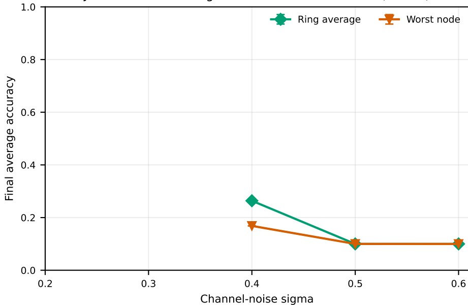
Joint SS+EBM average versus worst node: CART (nonIID)
