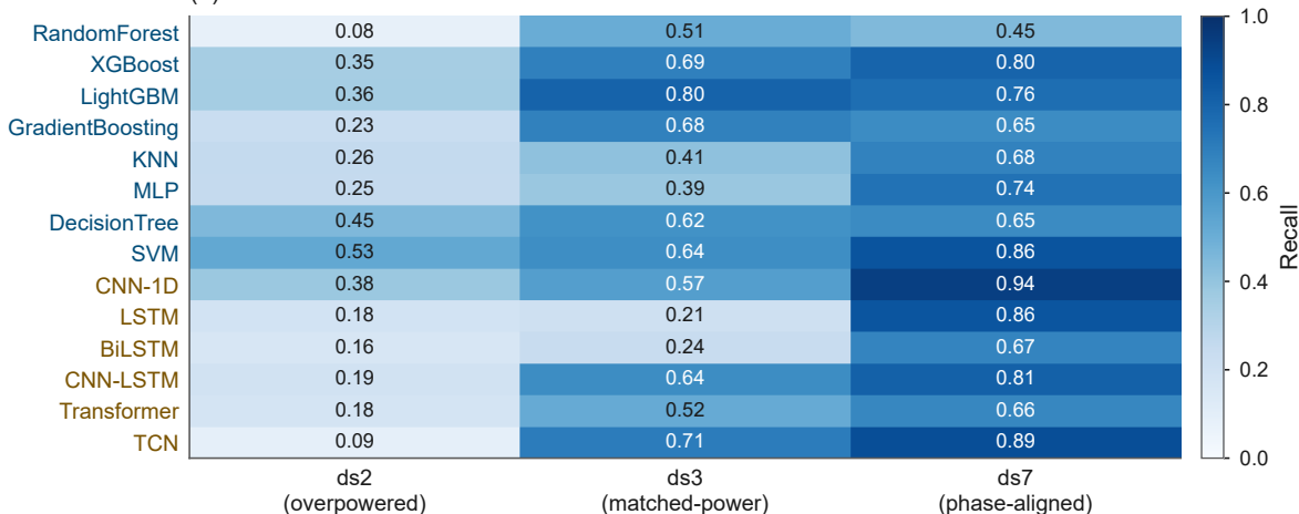
(a) Cross-scenario: detection recall on the held-out attack
