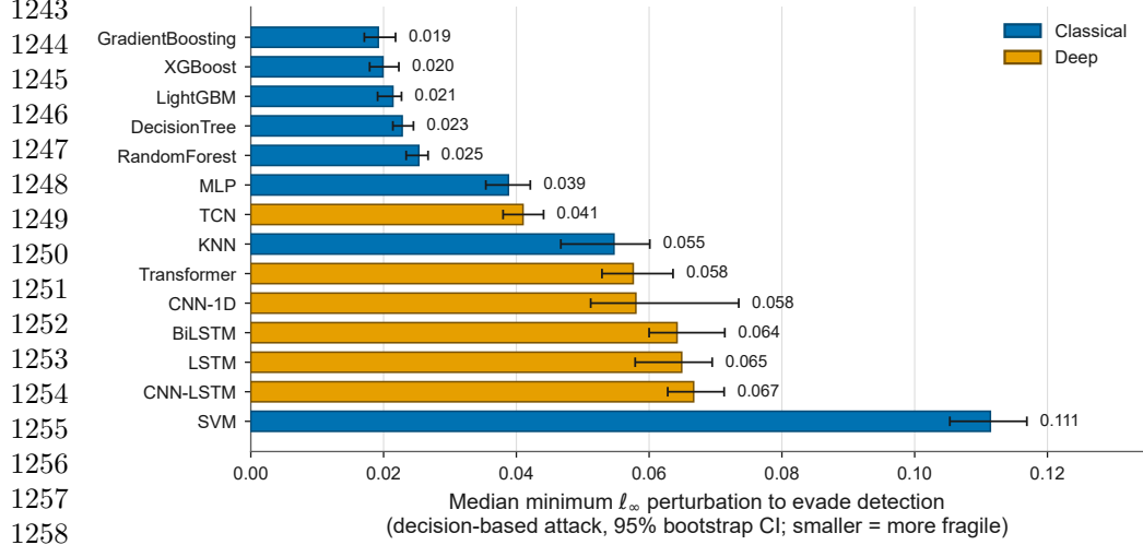
Fig. 8 Median minimum L_\infty perturbation needed to evade each detector under the gradient-free decision-based attack, with 95% bootstrap confidence intervals over the 500 attacked samples per detector. Smaller is more fragile. The five tree-ensemble classical detectors are the easiest to evade; the support-vector machine is the single robust outlier, needing roughly six times the perturbation of the most fragile detector. Within the tree cluster and within the nearest-neighbour/deep-model band the intervals overlap, so neither internal ranking is resolved.
