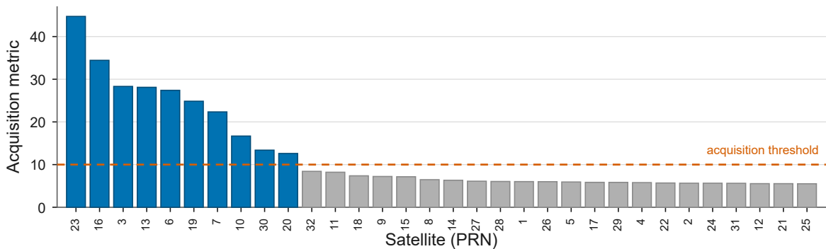
(b) Acquisition of PRN 23
