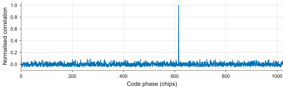
(b) Acquisition of PRN 23
