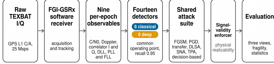
Fig. 1 Signal-level evaluation pipeline. Raw TEXBAT in-phase and quadrature recordings are processed by the FGI-GSRx software-defined receiver into per-epoch observables, which feed eight classical and six deep detectors. Every detector is placed at the common recall-0.95 operating point and attacked by the same suite, from white-box FGSM and PGD through multi-surrogate transfer and the GNSS domain attacks to the gradient-free decision-based attack.
