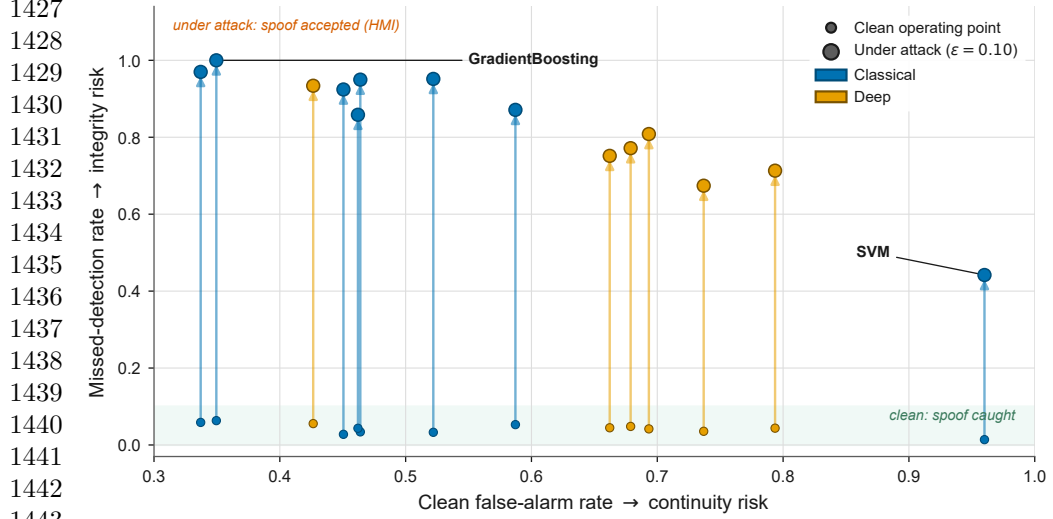
Fig. 12 Operational integrity view. Each detector is shown on the missed-detection against false-alarm plane at its clean operating point (small marker) and after a single decision-based attack at a fixed, physically small budget \varepsilon = 0.10 (about 6 dB of C/N_0 ; large marker), with the false-alarm rate held at its clean value because the evasion attack targets spoofed epochs. Missed detection is the integrity risk that precedes hazardously misleading information; the false-alarm rate is the continuity risk. Higher is worse on both axes, the reverse of clean F_1 in Figure 7: the gradient-boosting model, second best on clean detection, reaches the highest missed detection under attack, and the support-vector machine the lowest, so the ordering under attack does not follow clean performance (Figure 10). Every detector leaves the low-missed-detection band under the attack, and none remains in a region an integrity monitor could use.
