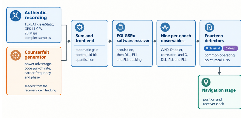
Fig. 2 How a transmitted attack becomes a detector input. A counterfeit GPS L1 C/A signal is generated as radio samples and added to authentic recorded samples. The sum passes through the front end and is tracked by the FGI-GSRx software receiver, which produces the nine per-epoch measurements the detectors read. The same tracking output also feeds the navigation stage, which yields the position and the receiver clock.
