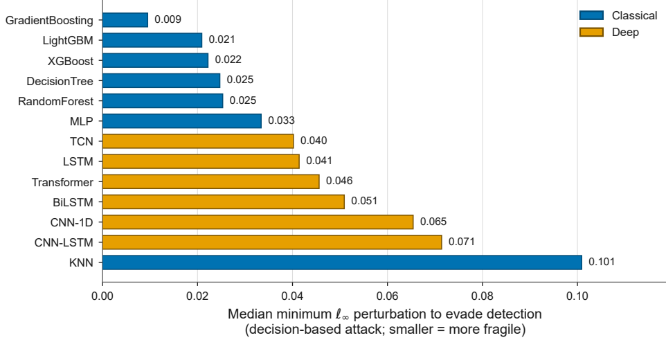
Fig. 8 Median minimum L_\infty perturbation needed to evade each detector under the gradient-free decision-based attack. Smaller is more fragile. The boosted-tree and tree detectors are the easiest to evade, the gradient-boosting model most of all despite its best clean F_1 , and the nearest-neighbour detector is the single robust outlier.
